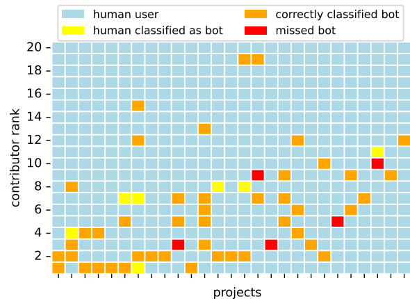
Figure 2: Rank of top 20 most active contributors in 27 popular open-source software projects.
