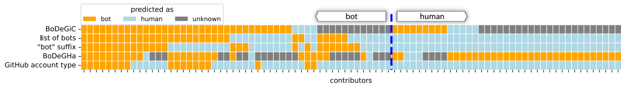
Figure 1: Classifications (“bot”, “human” or “unknown”) obtained from the five bot detection techniques. Only actual bots and humans wrongly classified as bot are displayed.
