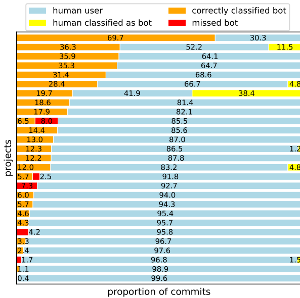
Figure 3: Proportion of commits made by the 20 most active contributors in each project
